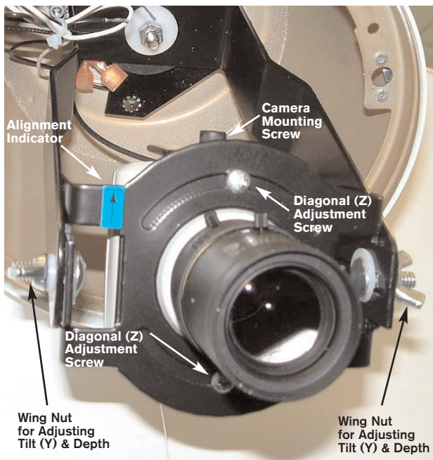
Figure 5: Camera/Lens Positioning
